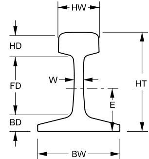
RAIL DIMENSIONS
